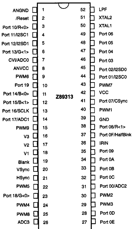
Figure 5. Z89313 52-Pin DIP
