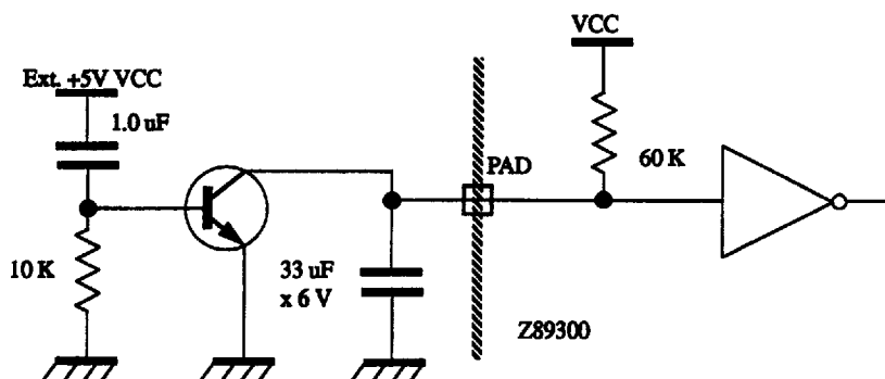
Figure 26. Reset Circuit
