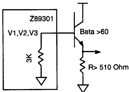
Figure 13. Recommended Circuit
