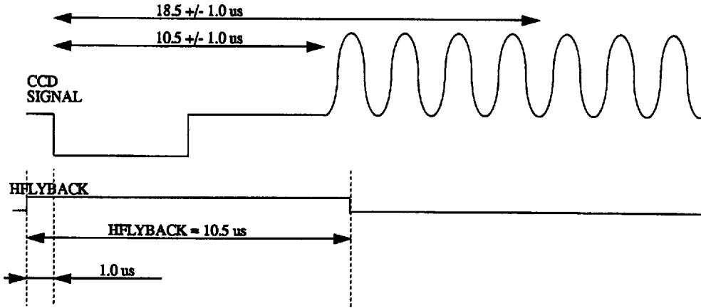
Figure 29. Register Settling Timing Diagram
