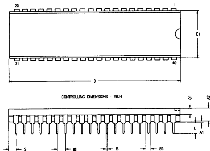
40-DIP Package Diagram
