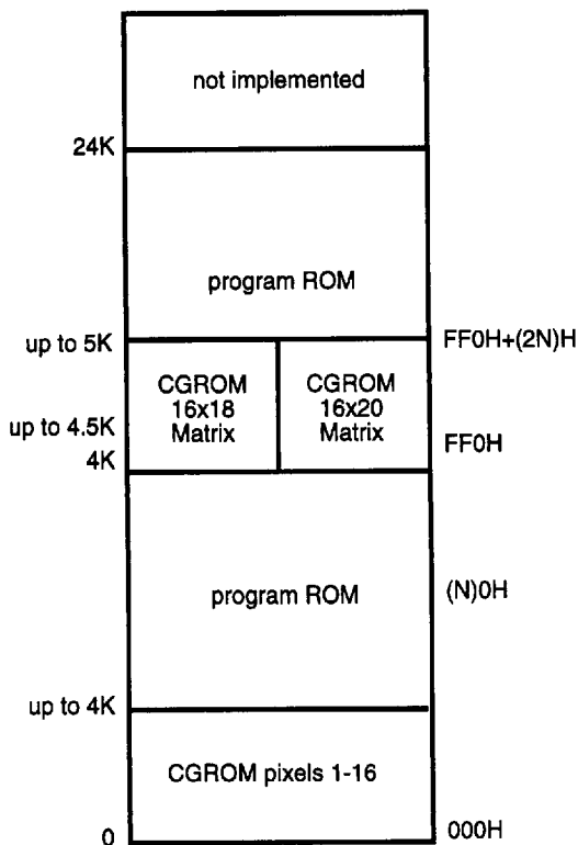
Figure 14. Program Read Only Memory
