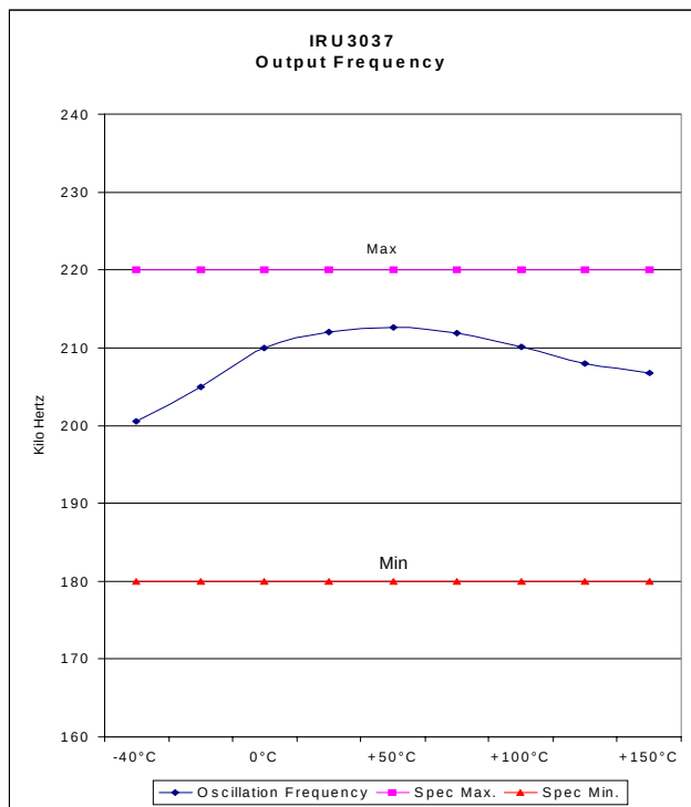
Figure 12 - Output Frequency
