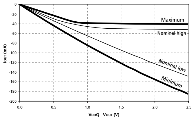
Figure 8: Pull-Up Characteristics
