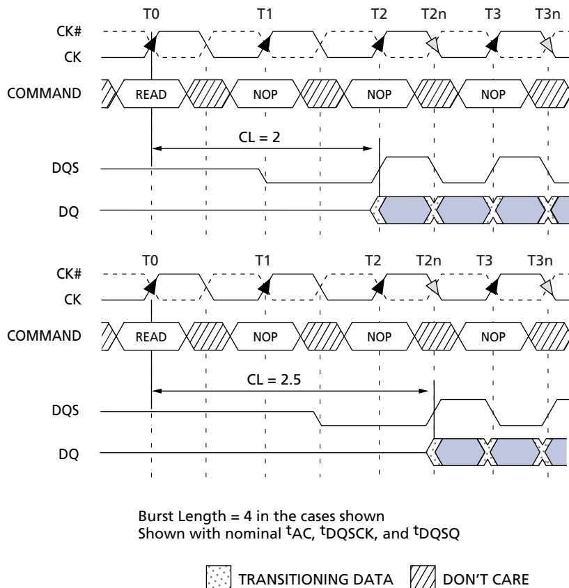
Figure 4: CAS Latency Diagram
