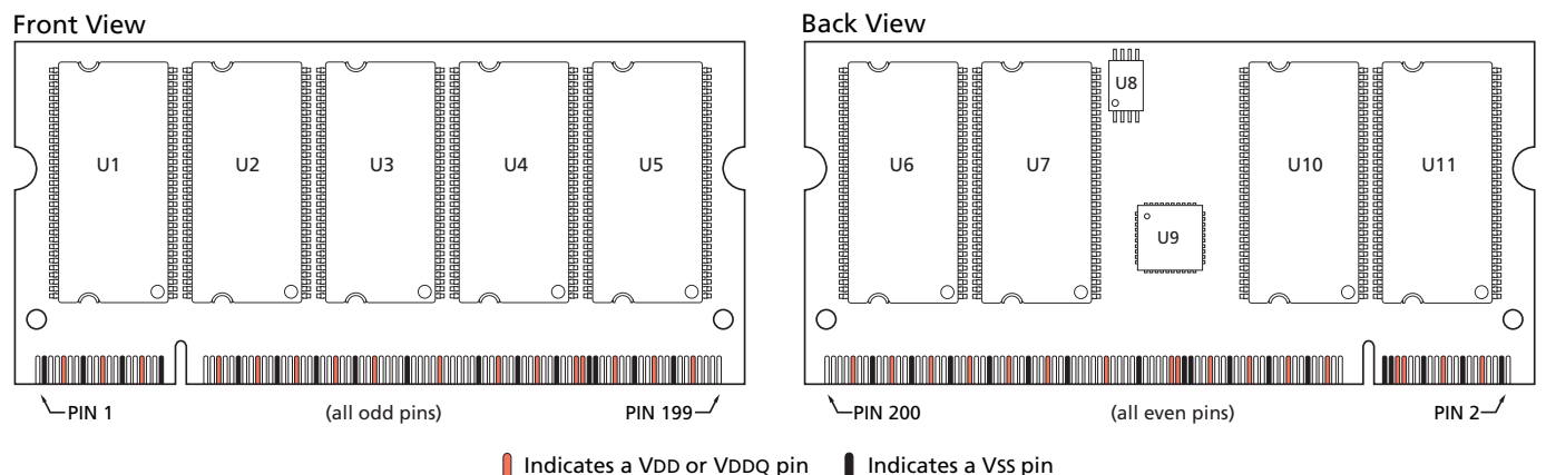
Figure 1: Module Layout
