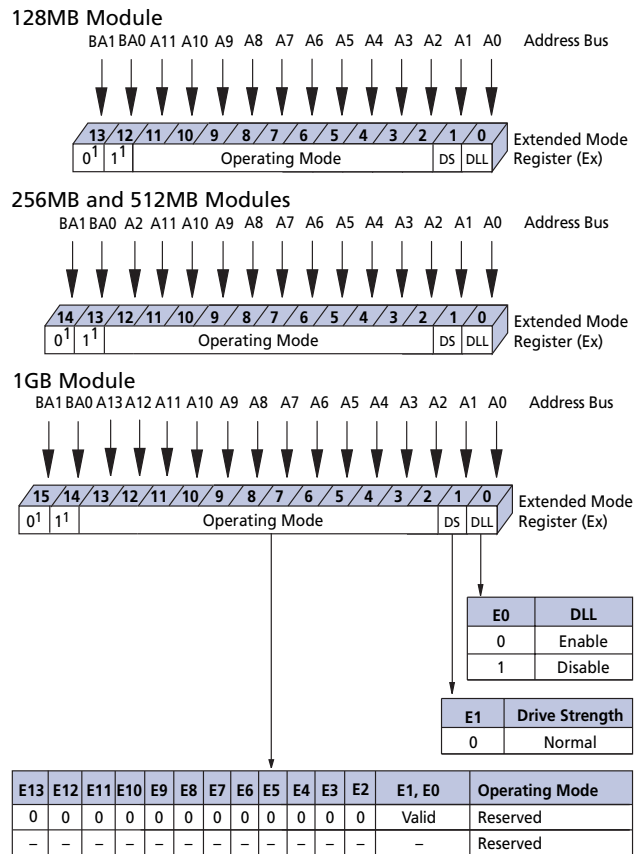
Figure 5: Extended Mode Register Definition Diagram
