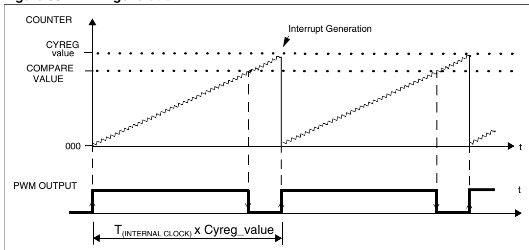
Figure 33. PWM generation
