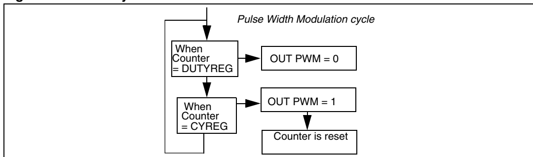
Figure 32. PWM cycle
