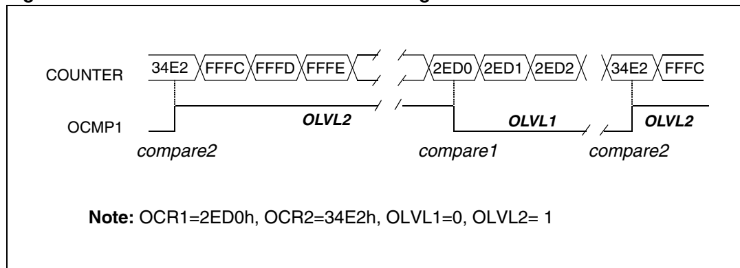
Figure 31. Pulse width modulation mode timing
