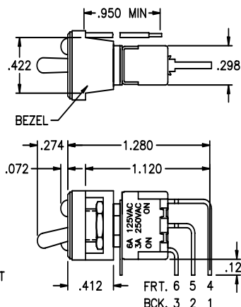
J95—TWO LED's
