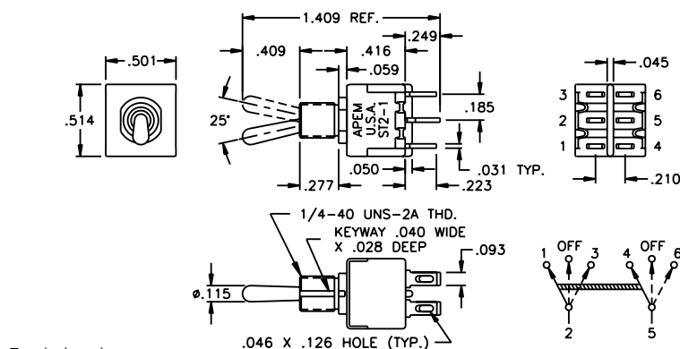
DOUBLE POLE
