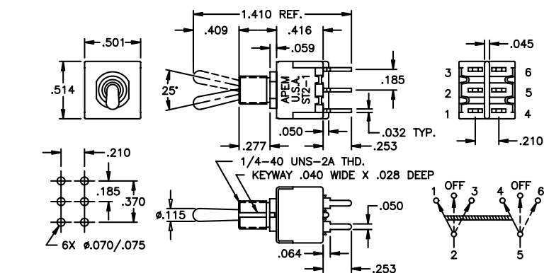
DOUBLE POLE
