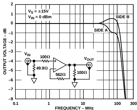
Figure 27. -3 dB Bandwidth vs. Frequency, G = +1
