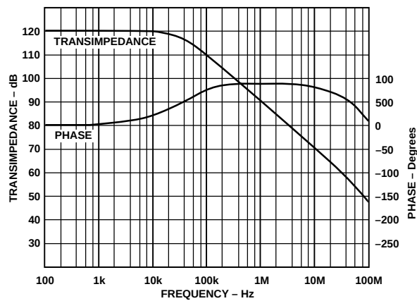
Figure 16. Open-Loop Transimpedance vs. Frequency
