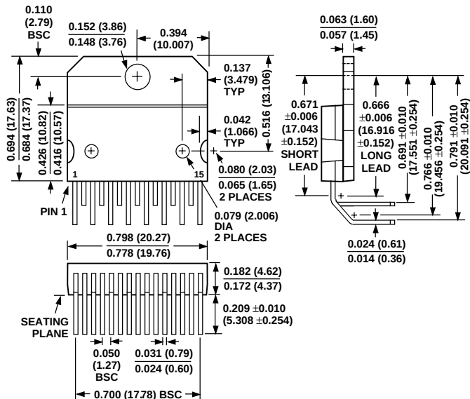
15-Lead Through-Hole SIP with Staggered Leads and 90° Lead Form (Y-15)
