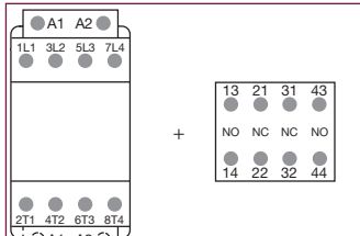
Combination 22 = AF09 ... AF38...-40-00 + CA4-22E
