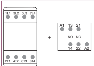
Combination 11 = AF09 ... AF38...-40-00 + CAT4-11E
