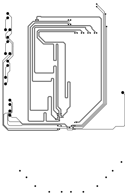
Figure 32. Si5110-EVB Layer 3—Signal Plane (Daughter Card)
