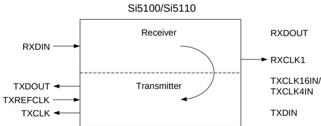
Figure 5. Line Loopback
