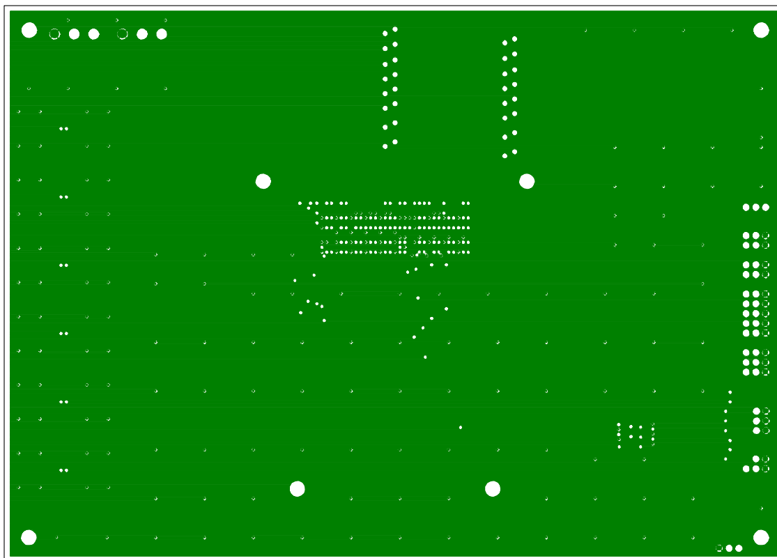
Figure 43. Layer 5—GND2 Plane (Loopback Motherboard)
