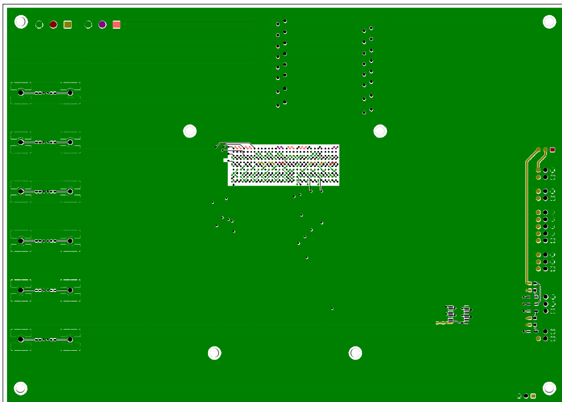
Figure 39. Layer 1—Component Side (Loopback Motherboard)
