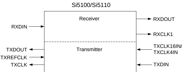
Figure 6. Full Duplex
