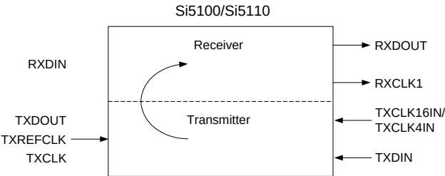
Figure 7. Diagnostic Loopback
