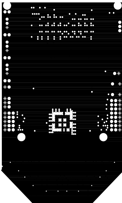
Figure 21. Si5100-EVB Layer 2—GND1 Plane (Daughter Card)
