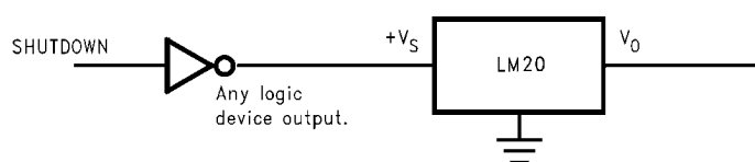
FIGURE 7. Conserving Power Dissipation with Shutdown
