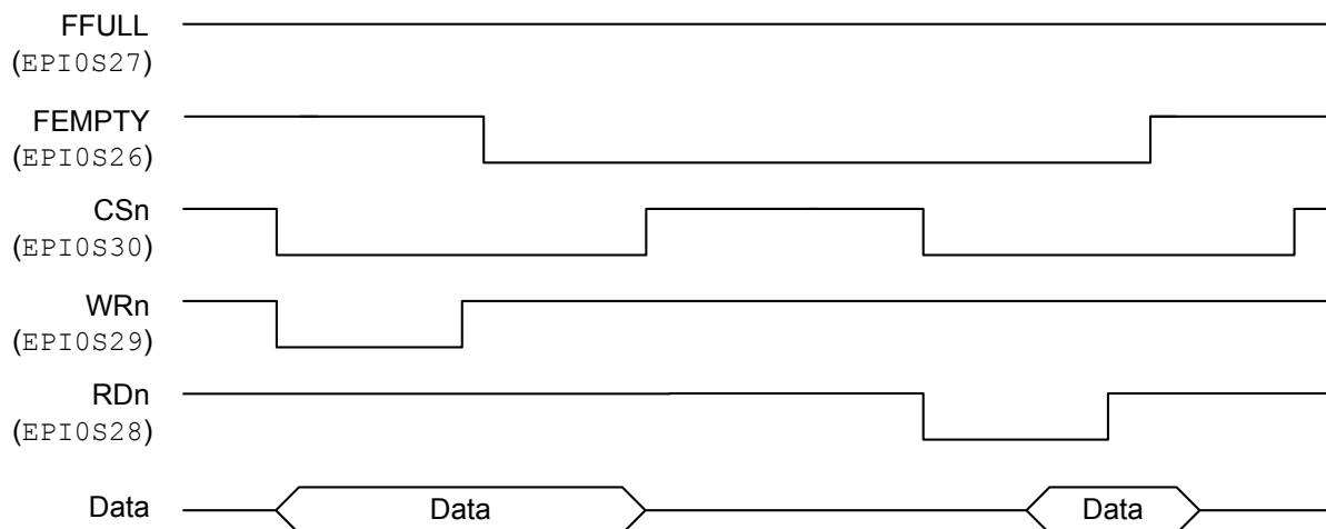
Figure 9-10. Two-Entry FIFO
