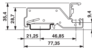
Dimensioned drawing
