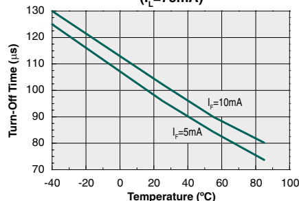
Typical Turn-Off vs. Temperature ( I_L=75\text{mA} )
