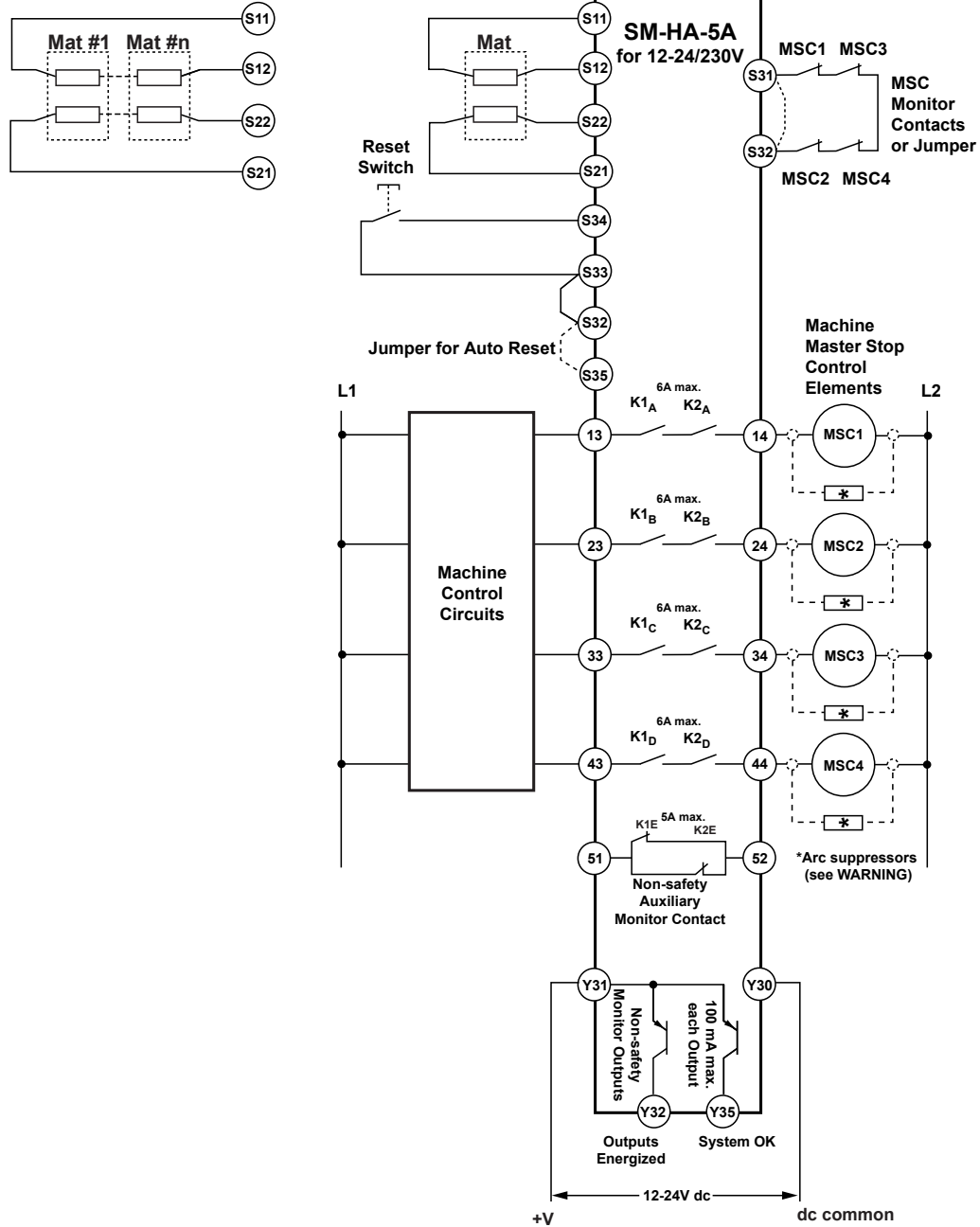
Figure 3. Hookup to a Four-Wire Safety Mat
