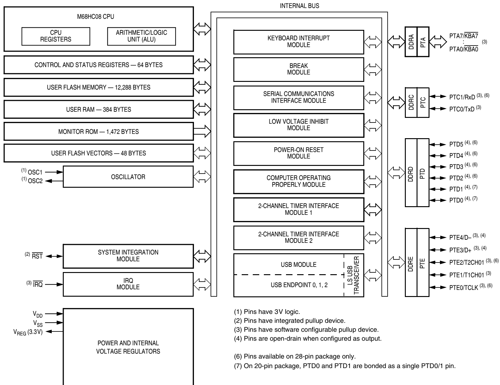
Figure 3. MC68HC908JB12 Block Diagram
