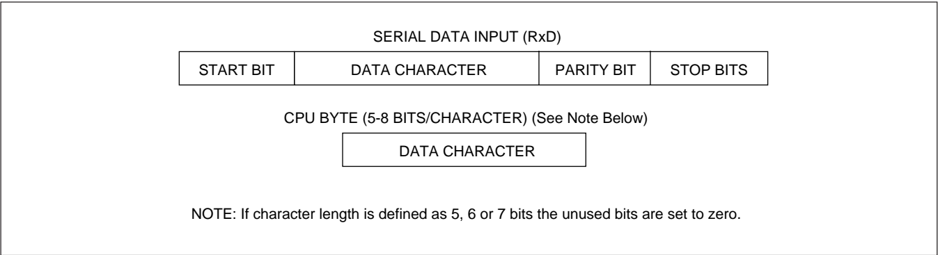
Figure 7: Receive Format
