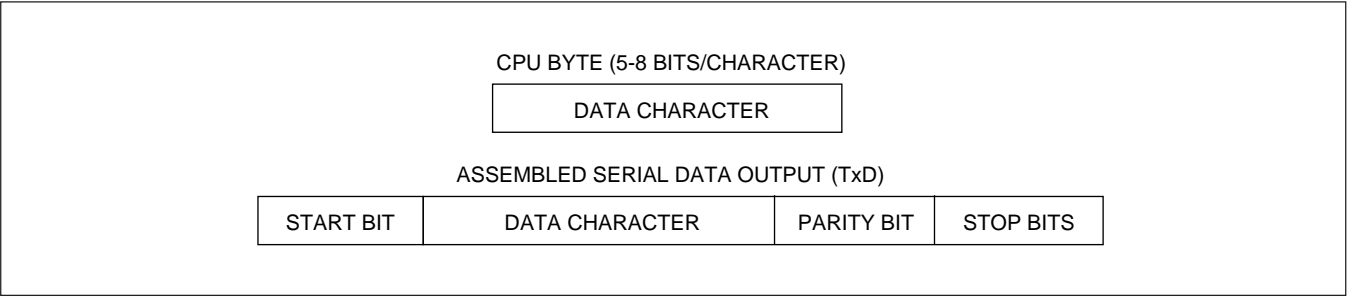
Figure 6: Transmission Format
