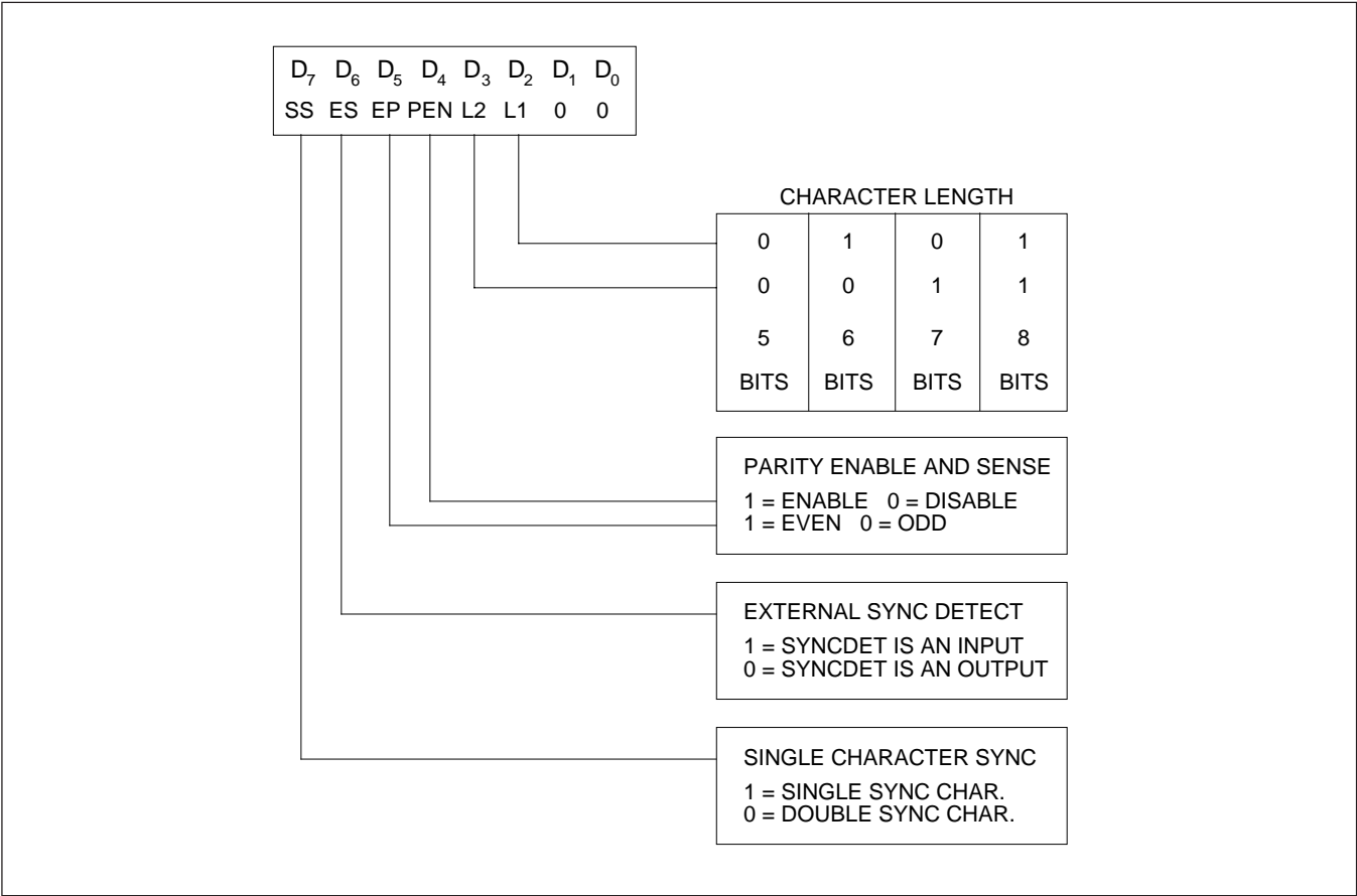
Figure 11: Mode Instruction Format, Synchronous Mode
