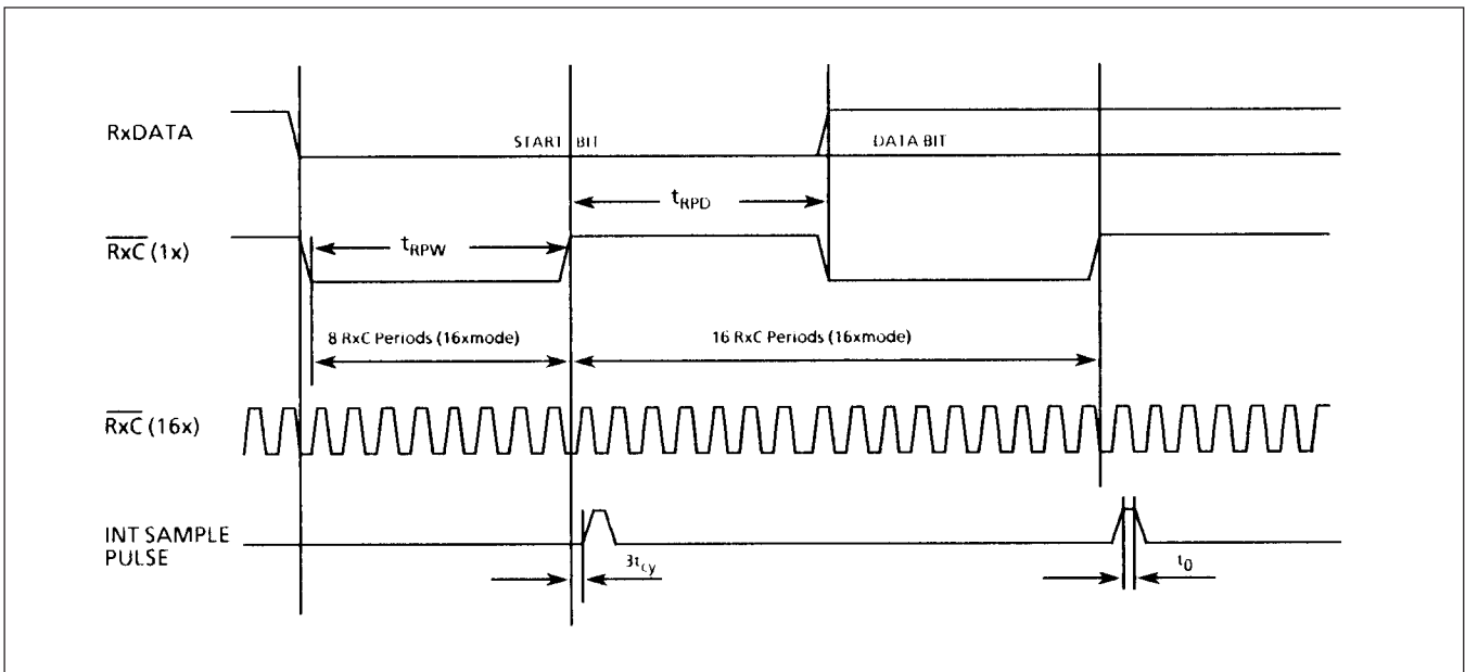
Figure 16: Receive Clock and Data
