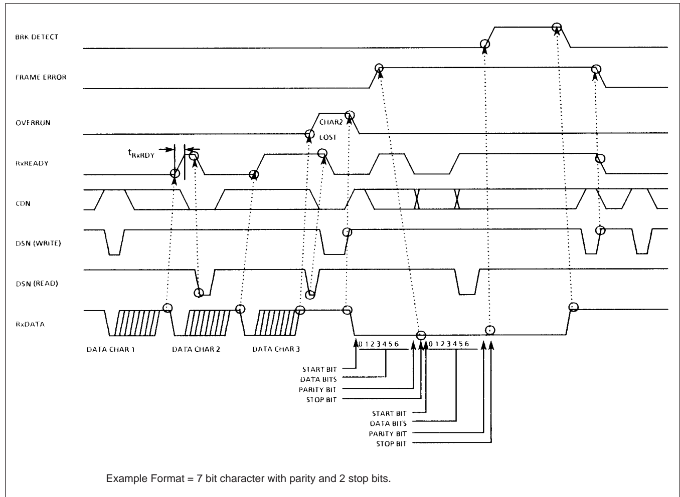
Figure 22: Receiver Control and Flag Timing (ASYNCR Mode)
