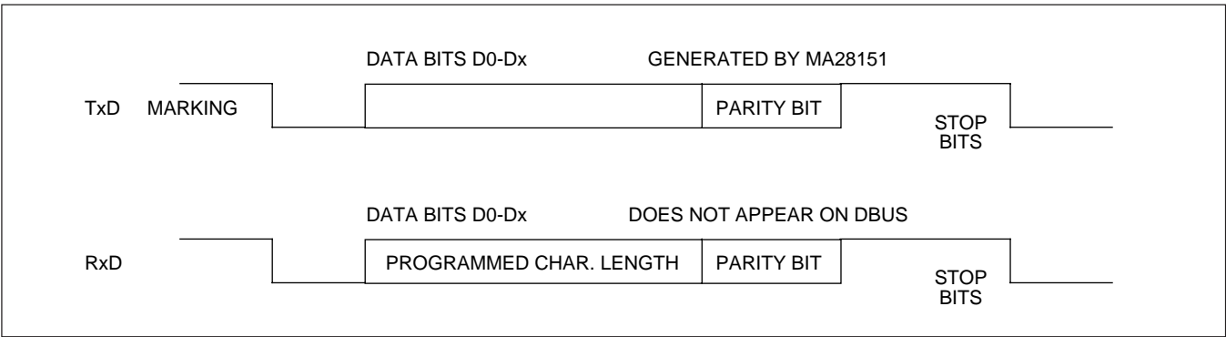
Figure 5: Asynchronous Mode
