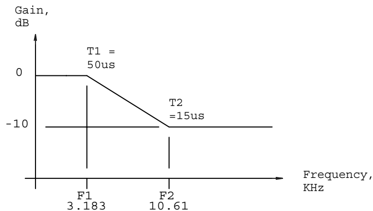
Figure 10. De-emphasis filter
