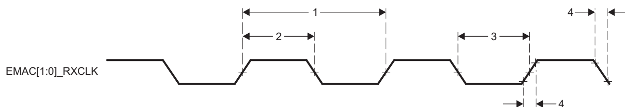
Figure 8-43. EMAC[1:0]_RXCLK Timing
