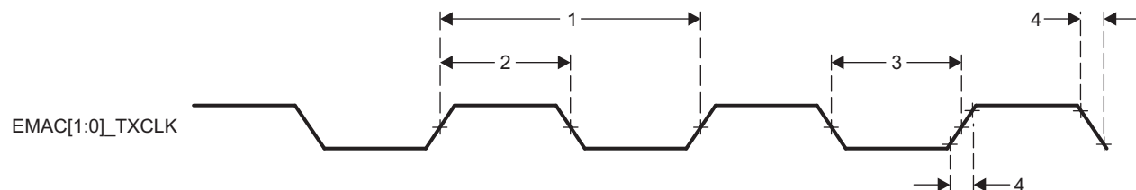
Figure 8-44. EMAC[1:0]_TXCLK Timing
