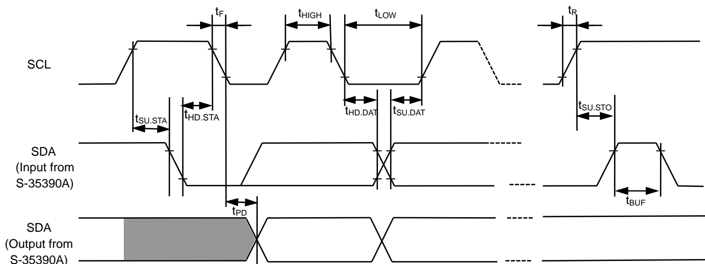
Figure 9 Bus Timing
