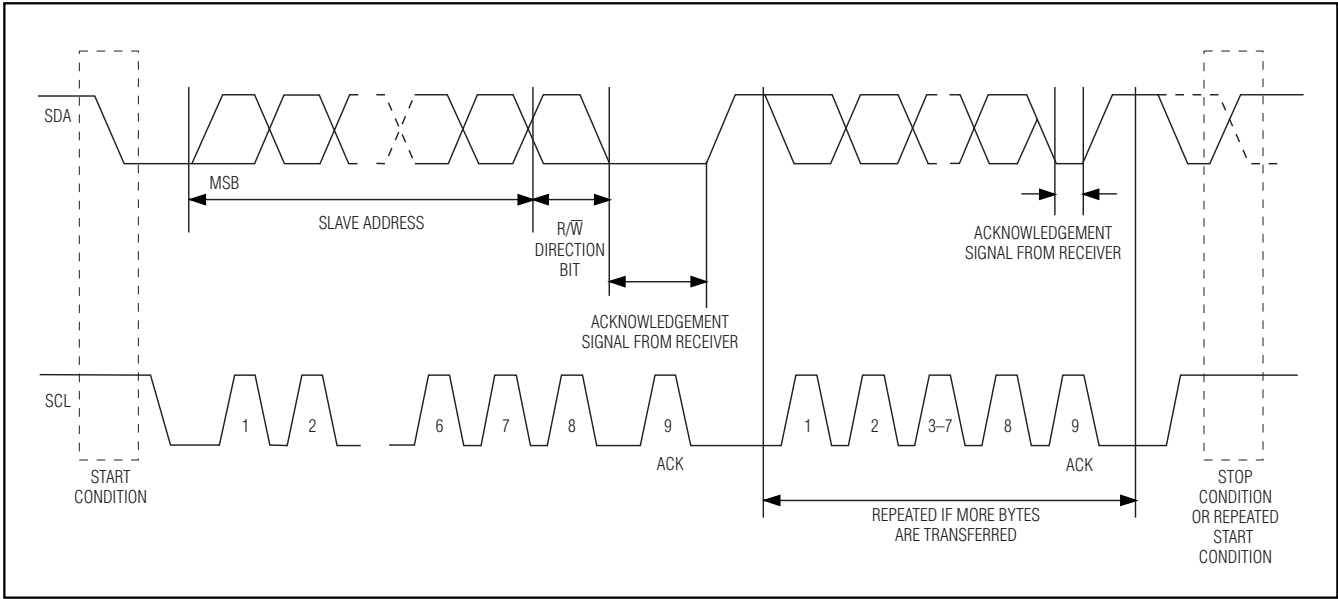
Figure 3. I²C Data Transfer Protocol
