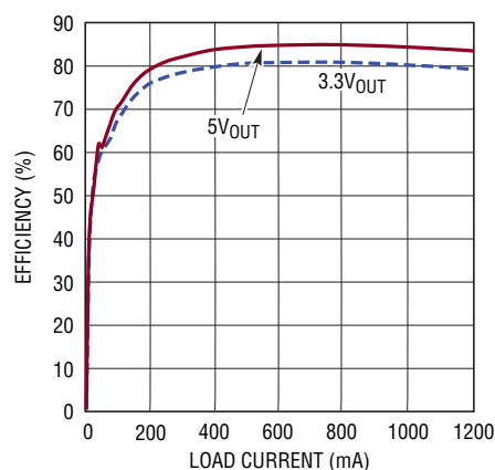
12V IN Efficiency (2MHz)
