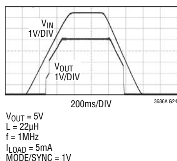
Start-Up Shutdown Waveform I_{LOAD} = 5mA
