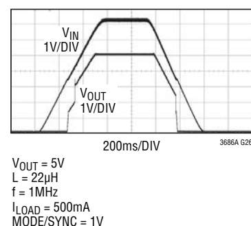
Start-Up Shutdown Waveform I_{LOAD} = 500mA
