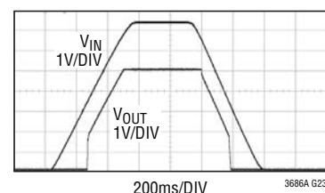
Start-Up Shutdown Waveform I_{LOAD} = 5mA
