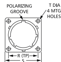
RECEPTACLE ASSEMBLY
