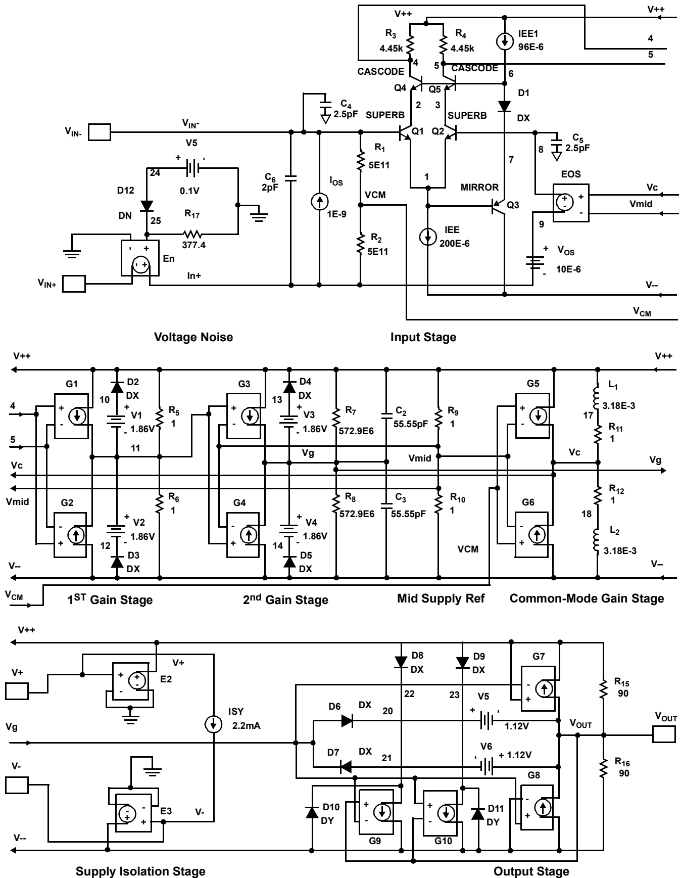
FIGURE 41. SPICE SCHEMATIC
