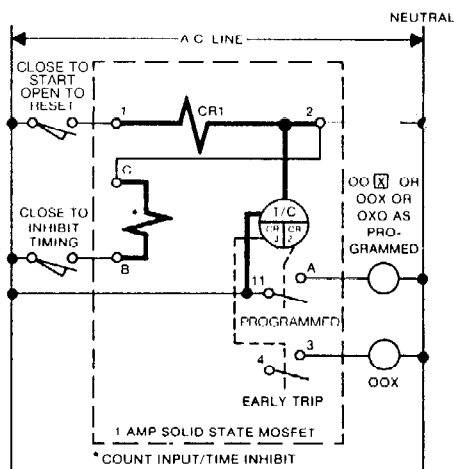
CX442A6 TIMER - SUSTAINED START INPUT
