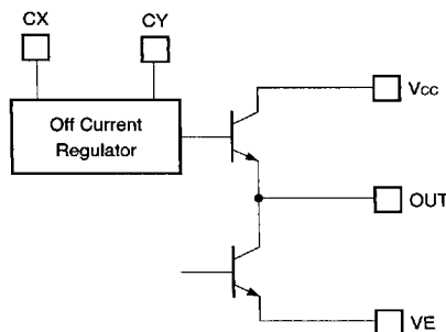
Output stage CH1, 2 equivalent circuit
