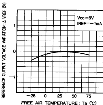
Fig.2 Reference voltage variation vs. ambient temperature
