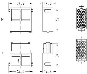
Contact arrangement view from termination side
