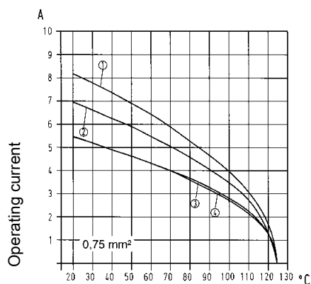
Ambient temperature
