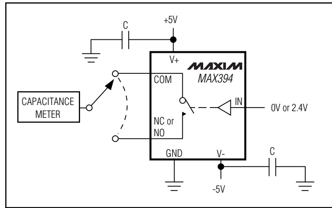
Figure 4. Channel On-Capacitance
