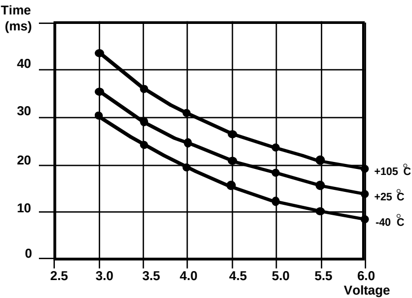
Figure 34. Typical WDT Time Out Period vs. V_{cc} Over Temperature
