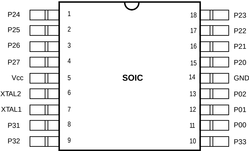
Figure 3. 18-Pin SOIC Pin Configuration
