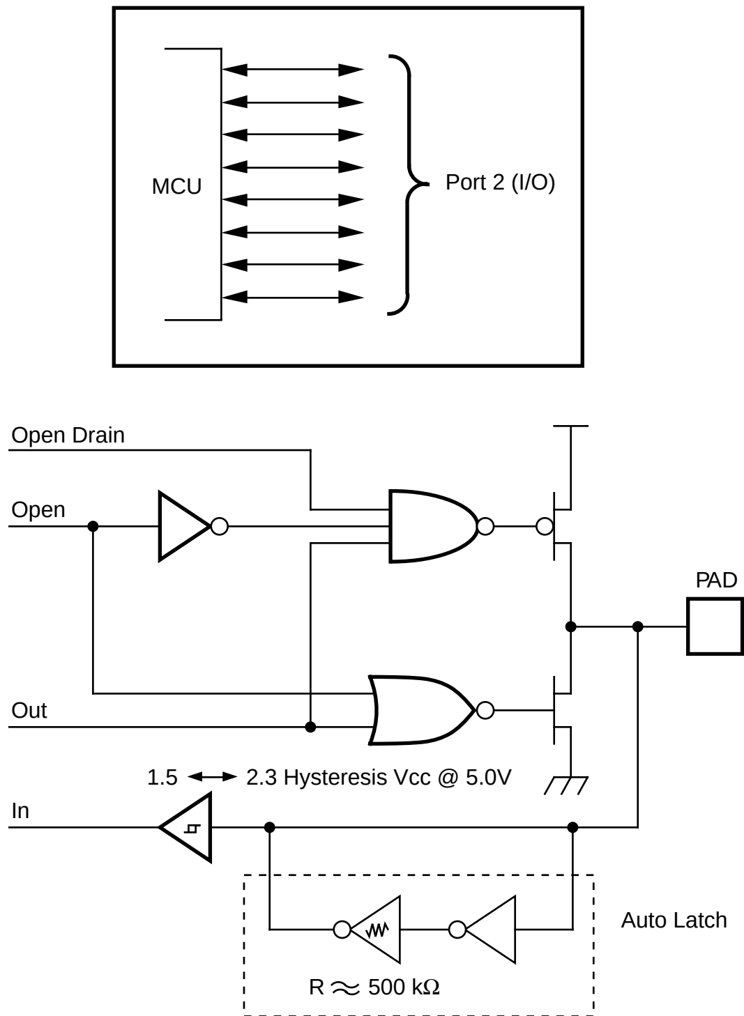
Figure 7. Port 2 Configuration
