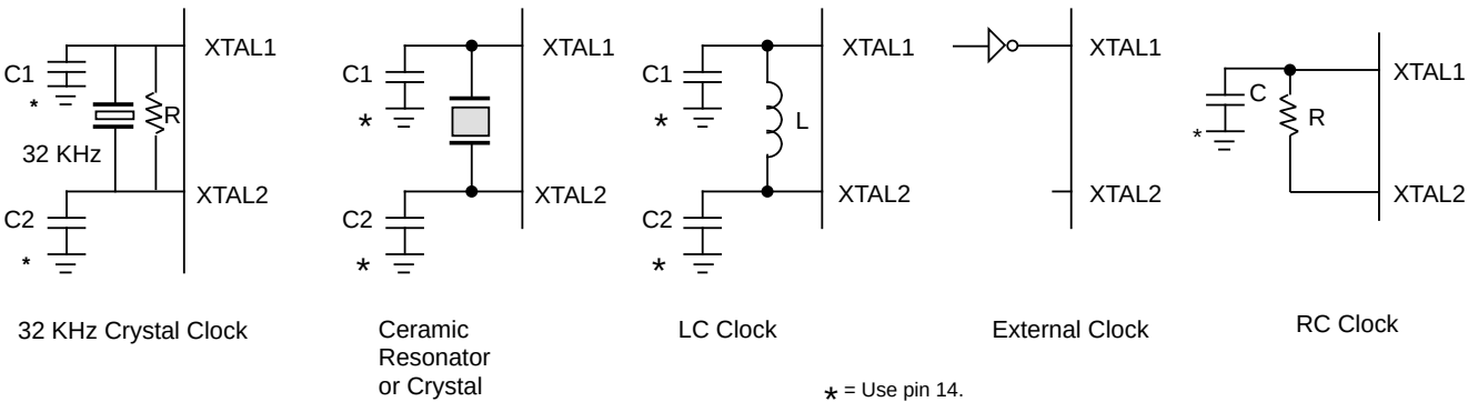
Figure 15. Oscillator Configuration
