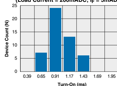
PAA140L Typical Turn-On Time (N=50 Ambient Temperature = 25°C) (Load Current = 200mADC; I_F = 5\text{mADC} )
