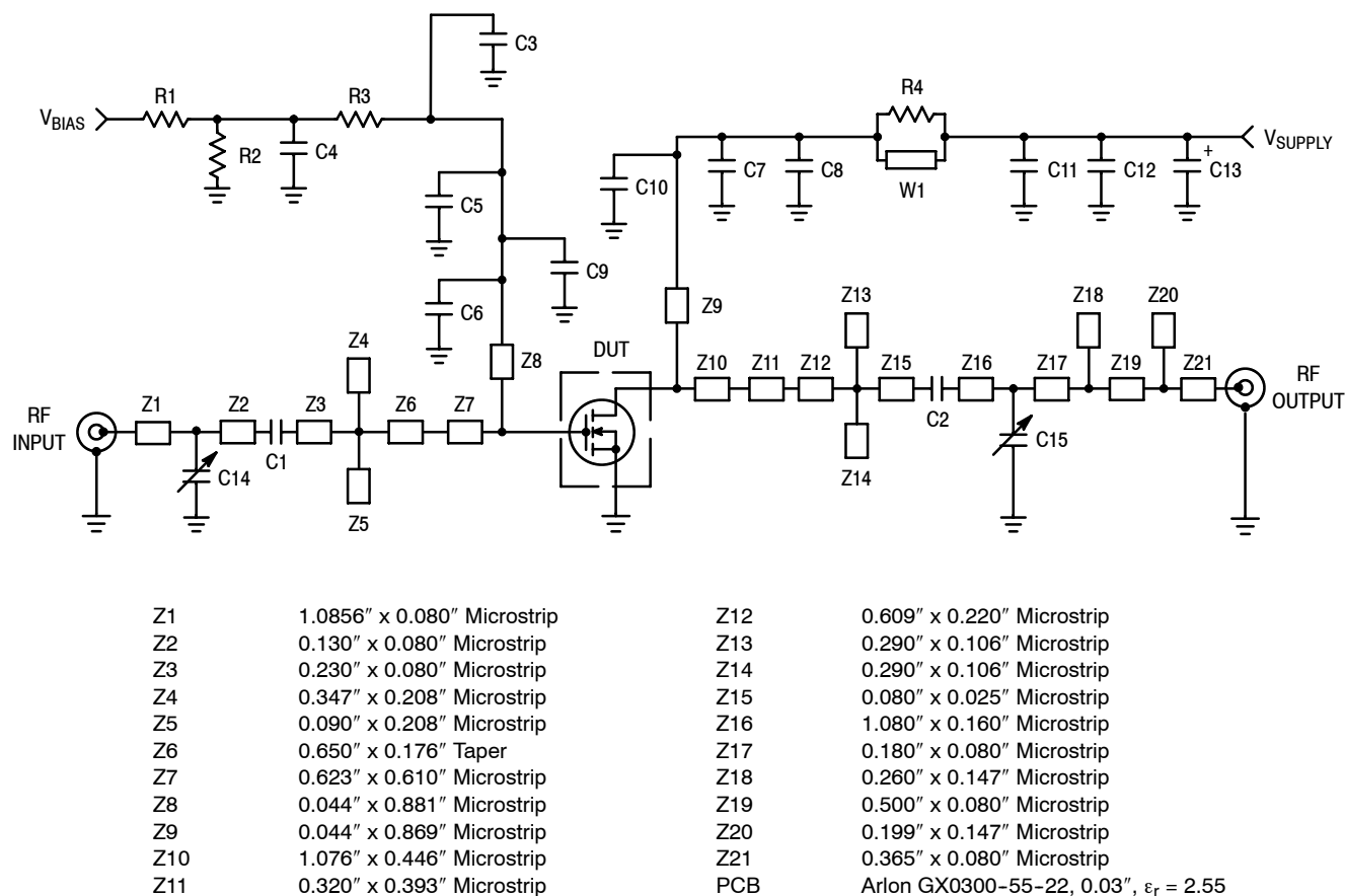
Figure 1. MRF5S21090HR3(HSR3) Test Circuit Schematic
