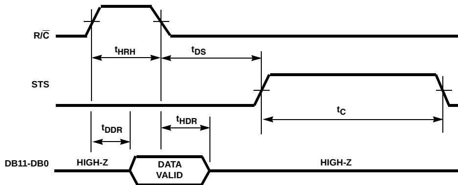
FIGURE 8. HIGH PULSE FOR R/\overline{C} - OUTPUTS ENABLED WHILE R/\overline{C} HIGH, OTHERWISE HIGH-Z
