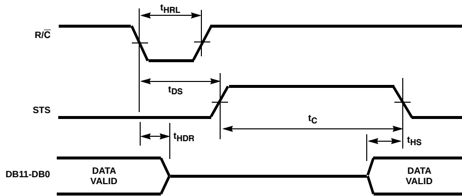
FIGURE 7. LOW PULSE FOR R/\overline{C} - OUTPUTS ENABLED AFTER CONVERSION
