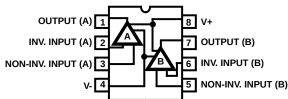
CA158, CA258, CA358, CA2904 (PDIP, SOIC) LM358, LM2904 (PDIP) TOP VIEW
