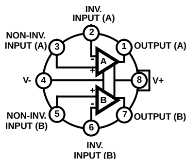
CA158, CA258, CA358 (CAN) TOP VIEW
