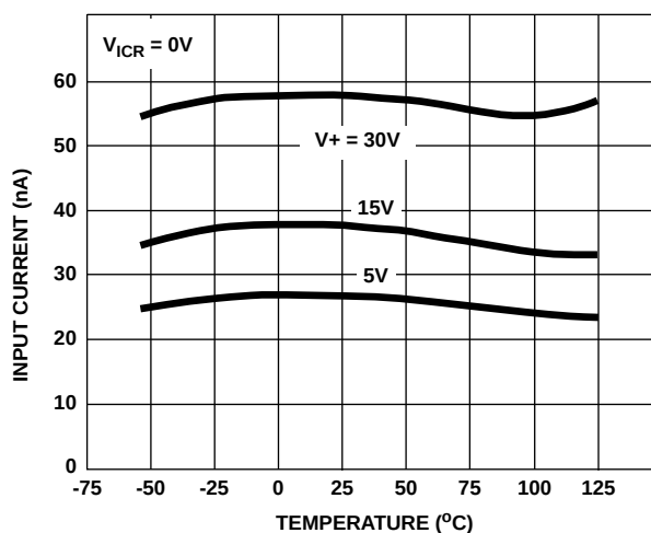
FIGURE 2. INPUT CURRENT vs AMBIENT TEMPERATURE
