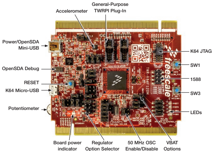
Figure 1: Front side of TWR-K64F120M
