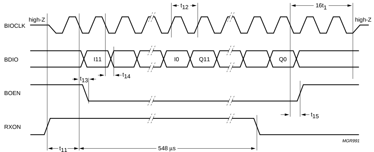
Fig.6 Timing of the baseband serial interface receive path; for the timing values see Table 5.
