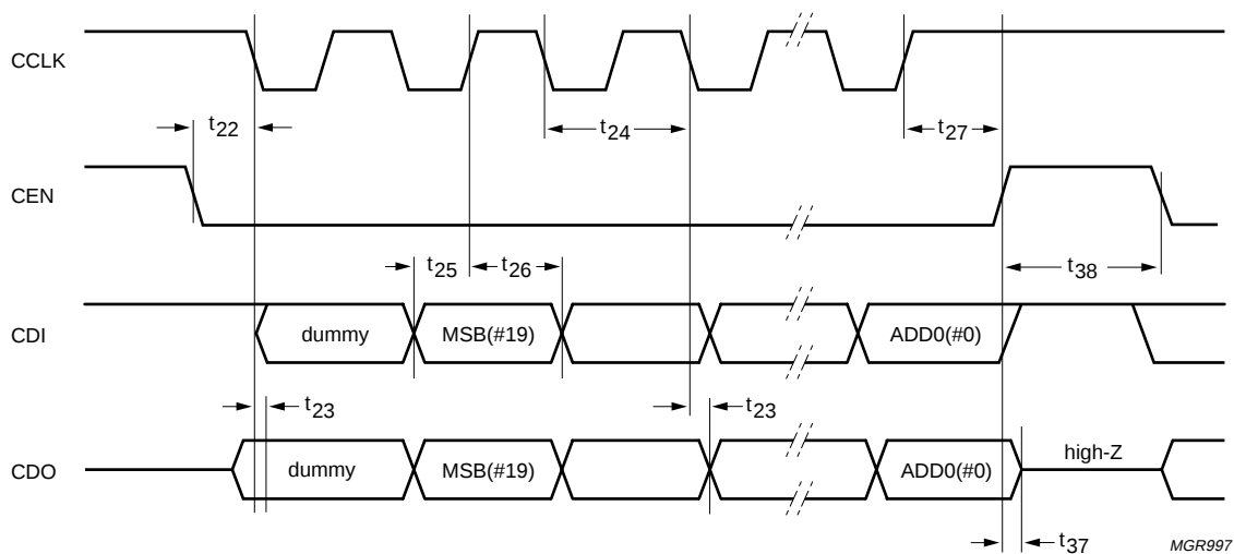
Fig.11 Timing diagram of the Control Serial Interface (CSI).
