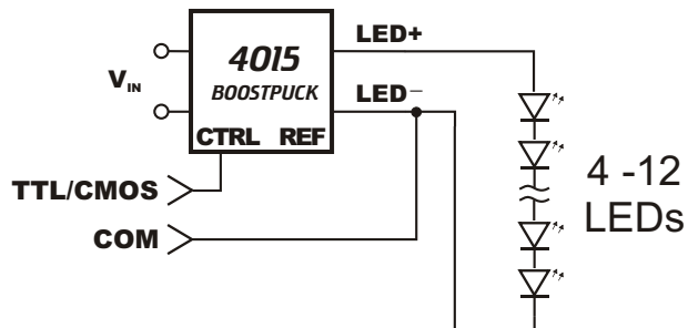
Figure 10. Pulse/Strobe input 5V=OFF
