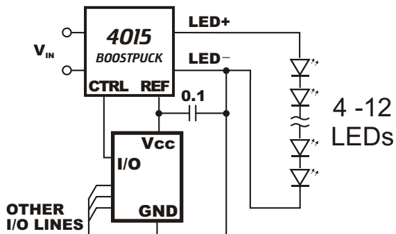
Figure 12. Interface to PIC or other microcontroller
