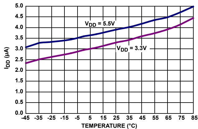
FIGURE 3. I_{DD3} vs TEMPERATURE
