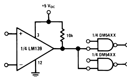
Driving TTL
