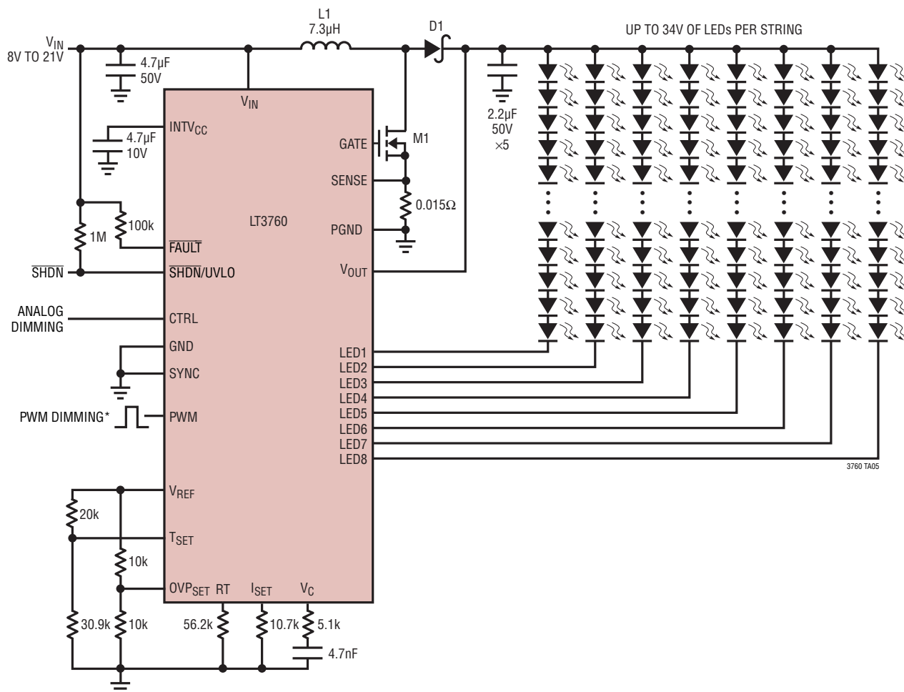
15W LED Driver, 750kHz Boost, 8 Strings, 55mA Per String
