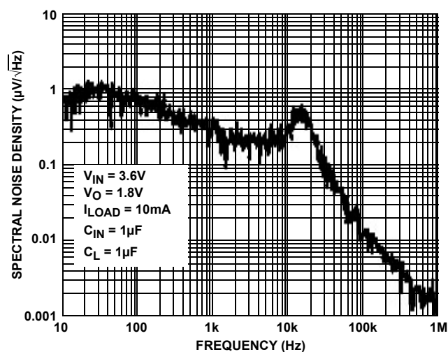
FIGURE 18. SPECTRAL NOISE DENSITY vs FREQUENCY
