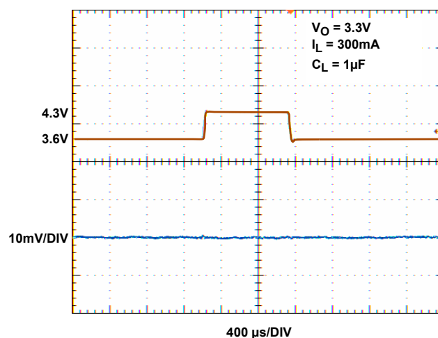
FIGURE 14. LINE TRANSIENT RESPONSE, 3.3V OUTPUT
