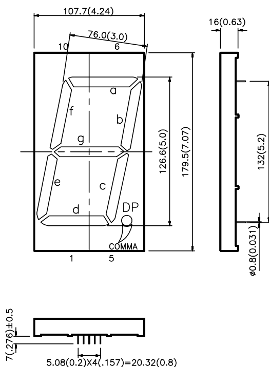
Package Dimensions
