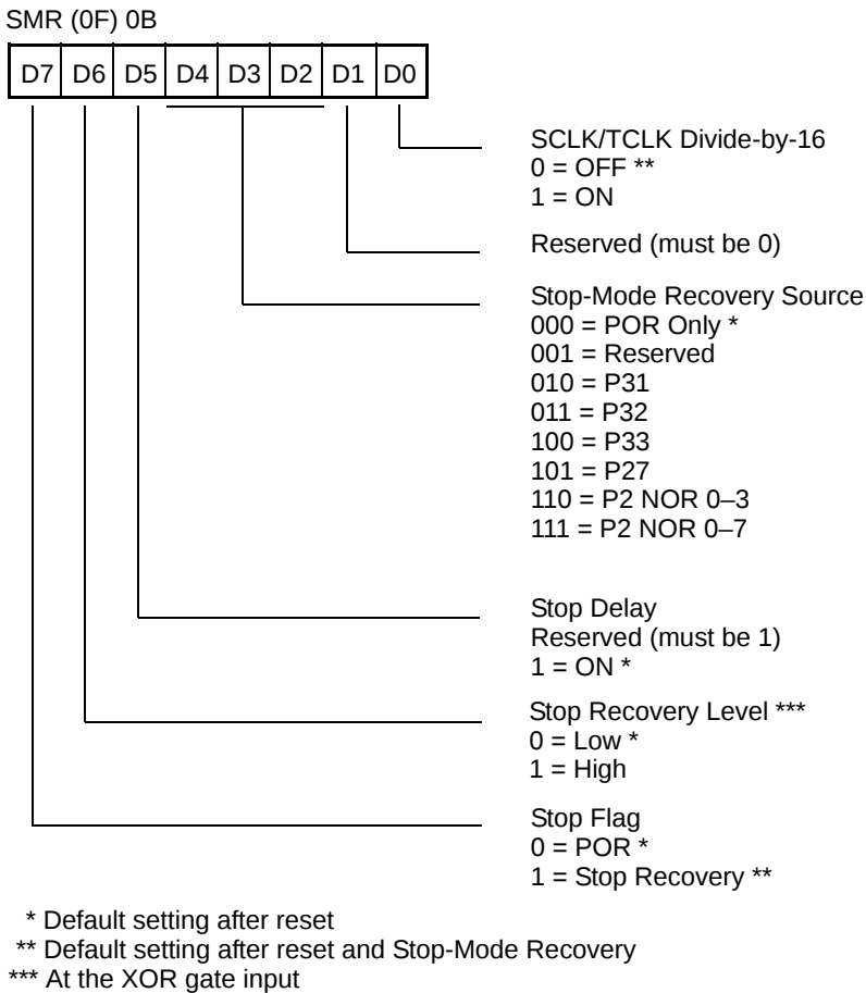
Figure 47. Stop-Mode Recovery Register
