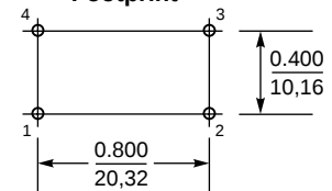
Footprint
