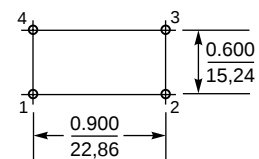
Footprint
