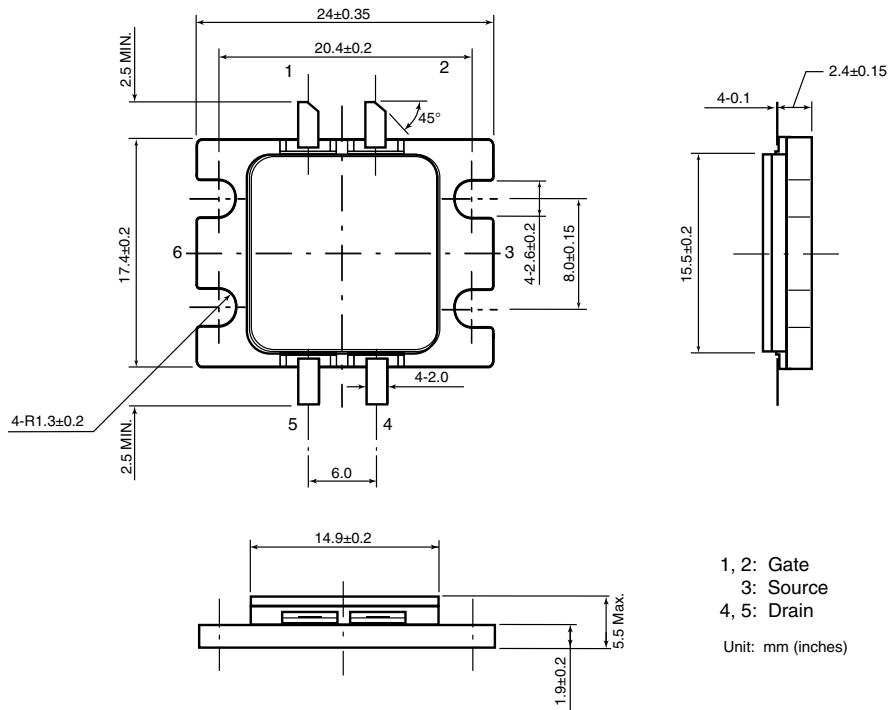
Case Style "IQ"
