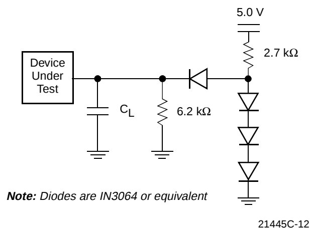
Figure 7. Test Setup
