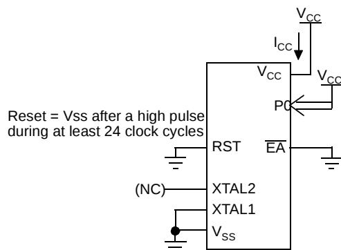
Figure 16. I_{CC} Test Condition, Power-down Mode
