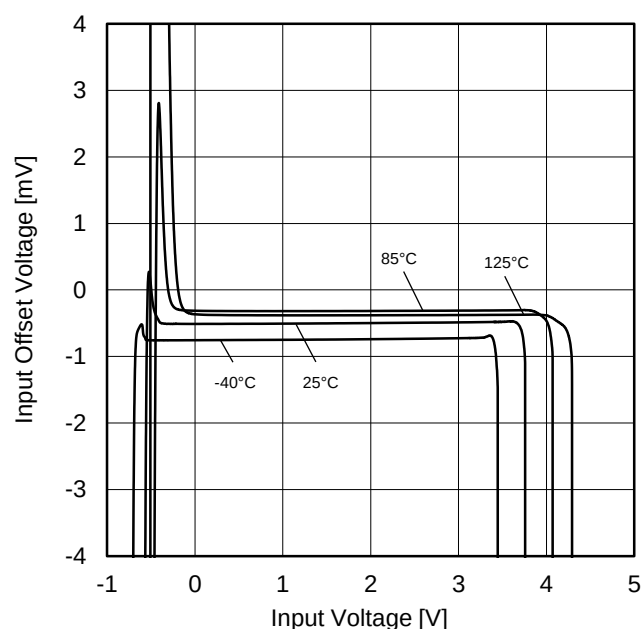
Figure 34. Input Offset Voltage vs Input Voltage ( V_{CC}=5V )
