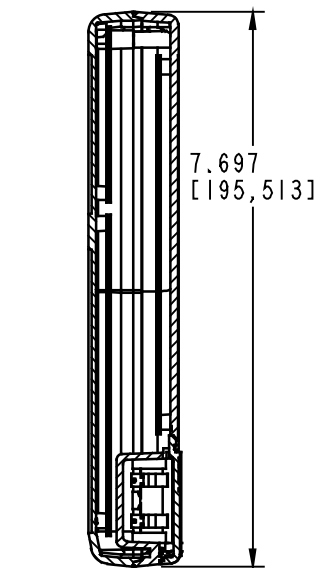
SECTION C-C
