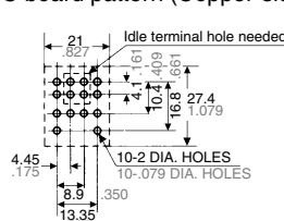
PC board pattern (Copper-side)
