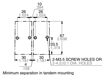
Chassis cutout
