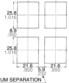
Chassis cutout
