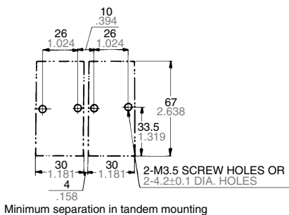
Chassis cutout
