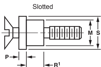
Threaded Retainer (see table)
