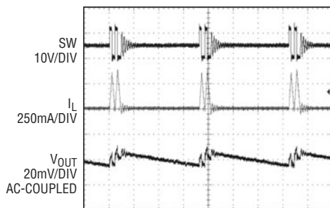
Output Voltage vs Time, Burst Mode Operation
