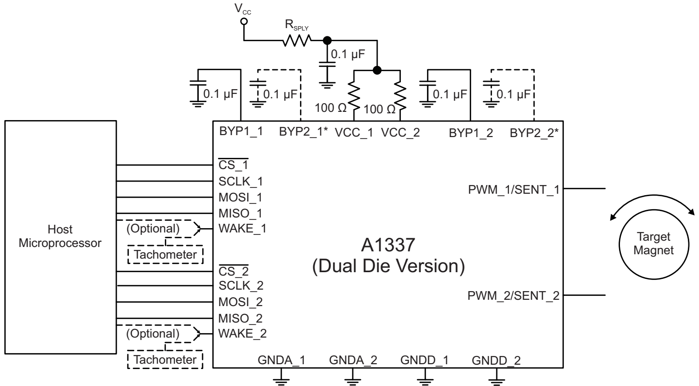
Figure 24: Typical application diagram (dual-die version) with EMC suppression resistor, R_{SPLY} , on supply line.
