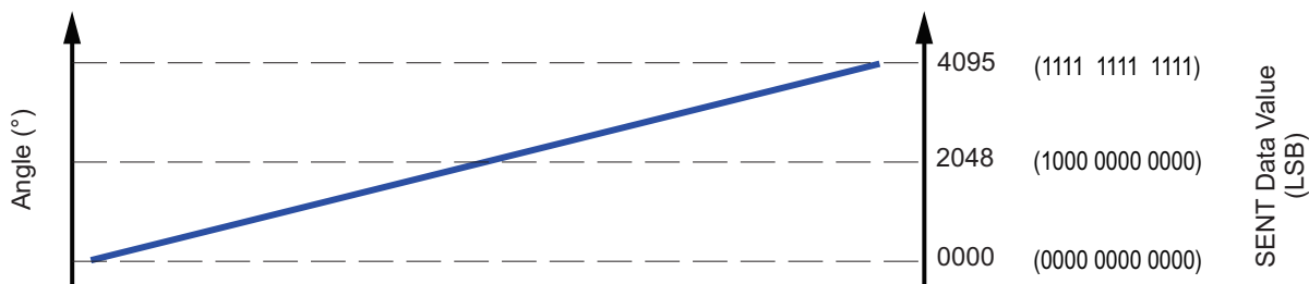
Figure 6: Angle is represented as a 12-bit digital value.
