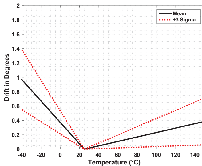
Figure 17: Angle Drift Relative to 25°C (300 G)
