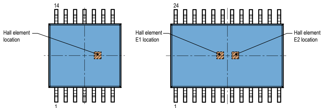
Figure 25: Hall element located off-center within the device body; refer to the Package Outline Drawing for reference dimensions
